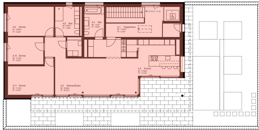
aGF Attika
